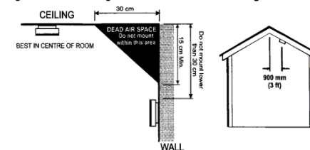
Figure 3i - Positioning the smoke/heat detector Figure 3ii
